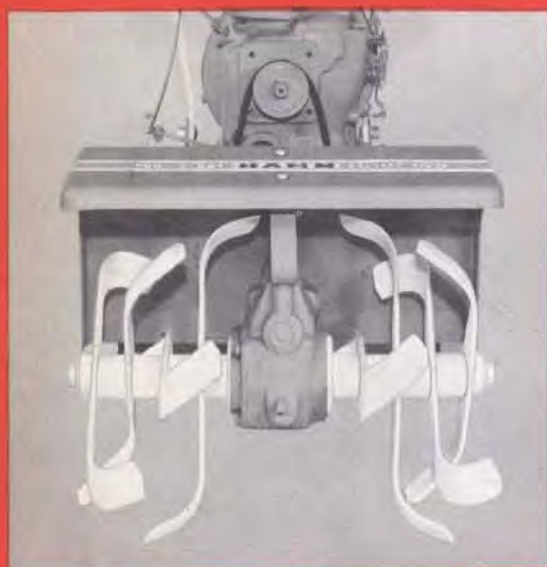
Tills or cultivates a full 17" swath; with Extension Tines added gives a wide 26" coverage.
